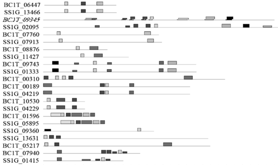
Fig. 2 CCCH zinc finger genes structures from and
