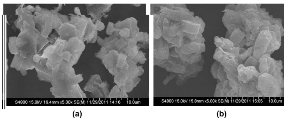
Fig. 1. The SEM partners of ZSM-5 and Fe-ZSM-5. (a) The SEM partners of ZSM-5 and (b) The SEM partners of Fe-ZSM-5.
